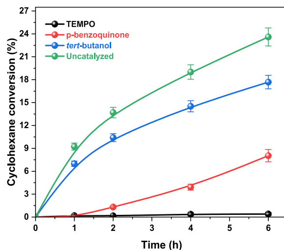
Figure 3. Conversion-reaction time profiles of the radical scavenging experiments in the uncatalyzed reaction. Reaction conditions: 130\text{ }^\circ\text{C} , 1.00 mol/L cyclohexane, 15 bar \text{O}_2 , 600 rpm, 6 h, 2 mol % of radical scavenger, acetonitrile as solvent, and biphenyl as the internal standard.
