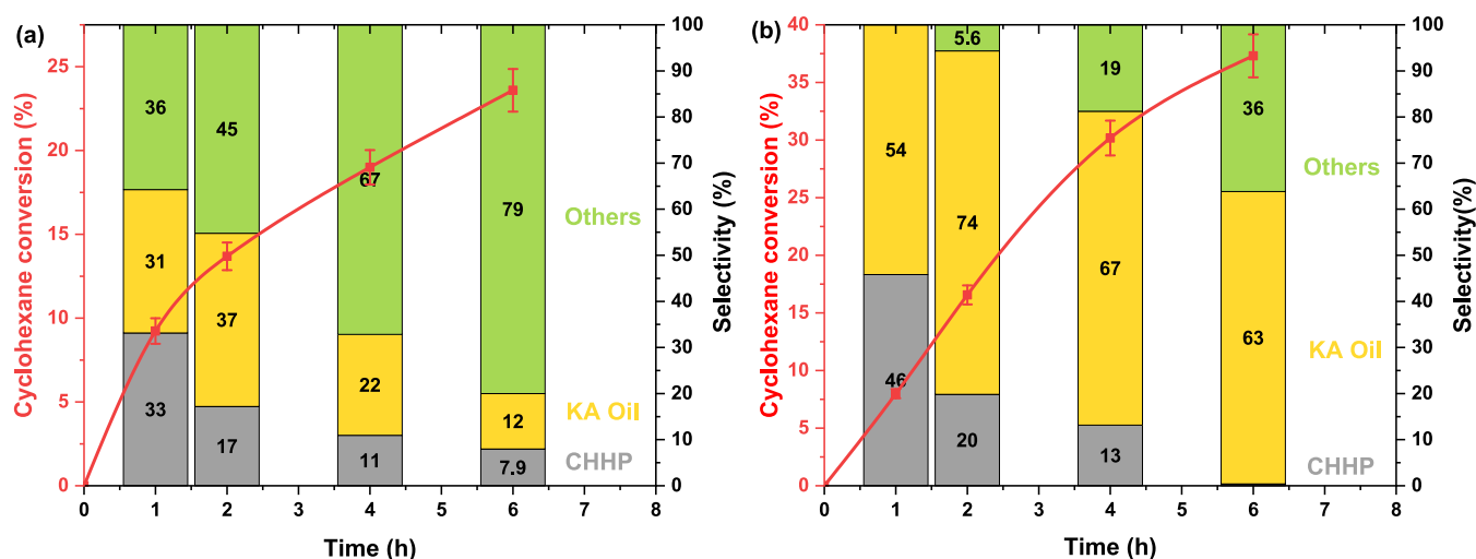
Figure 1. Conversion-selectivity profiles of the (a) uncatalyzed reaction and (b) catalyzed reaction using 20 mg \text{LaCo}_{0.7}\text{Fe}_{0.3}\text{O}_3 . Reaction conditions: 130 °C, 1.00 mol/L cyclohexane, 15 bar \text{O}_2 , 600 rpm, 6 h, acetonitrile as solvent, and biphenyl as internal standard.
