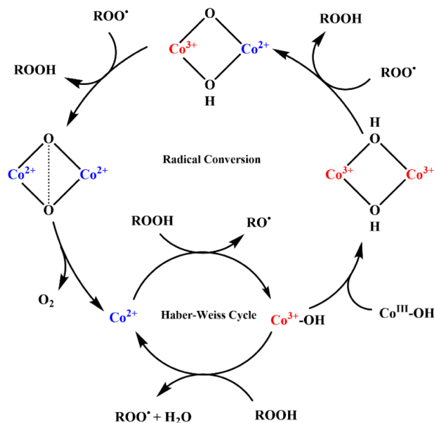
Figure 14. Postulated catalytic cycle for rapid conversion of highly oxidizing C 6 H 11 OO• to CHHP via Co-based oxyhydroxy moieties.
