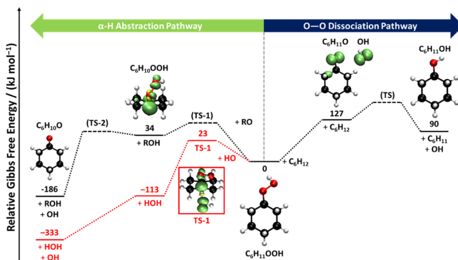
Figure 15. Energy diagram for the \alpha -H abstraction (left) vs O–O dissociation (right) pathways of CHHP ( C_6H_{11}OOH ). For the \alpha -H abstraction, paths for R = C_6H_{11}O (black) and R = H (red) are included. Verified transition states (TS) are shown as solid lines and hypothesized ones as dashed lines. The electron spin density is included as contour lines (plotted at isovalues of \pm 0.01 ). All energies refer to relative Gibbs free energies in solution in 95 mol % acetonitrile at 130 °C with 5 mol % of C_6H_{12} .
